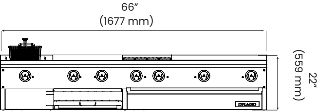
Vista frontal
